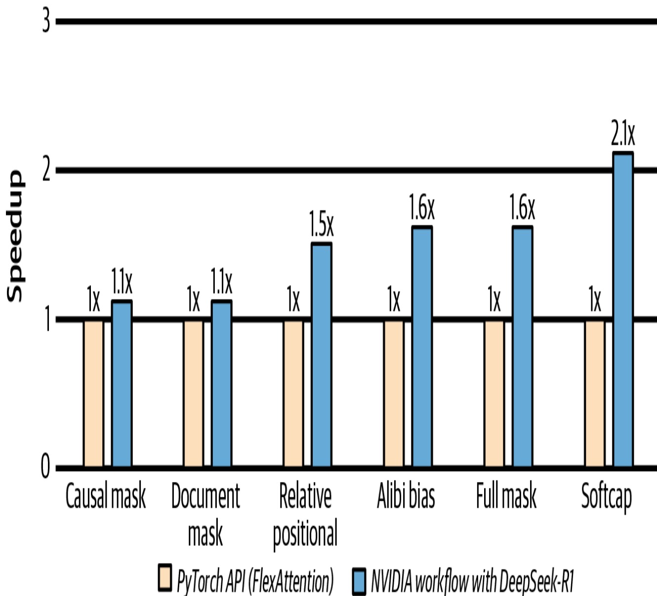
Figure 20-4. Automatically generated attention kernels achieved 1.1\times – 2.1\times speedups compared to PyTorch FlexAttention (source: Automating GPU Kernel Generation with DeepSeek-R1 and Inference Time Scaling | NVIDIA Technical Blog)
