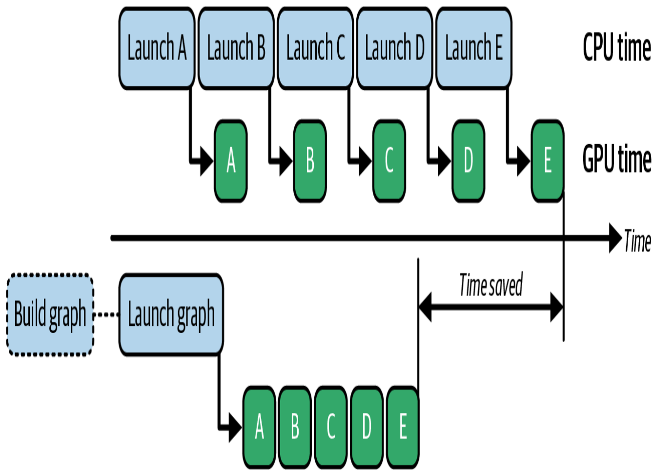
Figure 20-7. Graph execution in CUDA reduces overhead when launching multiple kernels in a sequence (source: https://oreil.ly/kxSDm )
