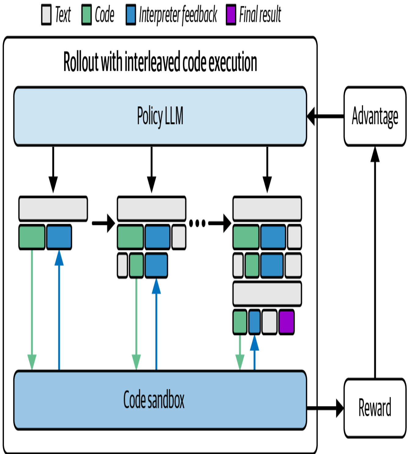
Figure 20-1. Using reinforcement learning to find the most optimal GPU kernel code for your environment
