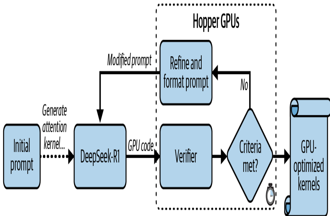
Figure 20-3. Inference-time scaling with DeepSeek-R1 on the NVIDIA Hopper platform (source: Automating GPU Kernel Generation with DeepSeek-R1 and Inference Time Scaling | NVIDIA Technical Blog )
