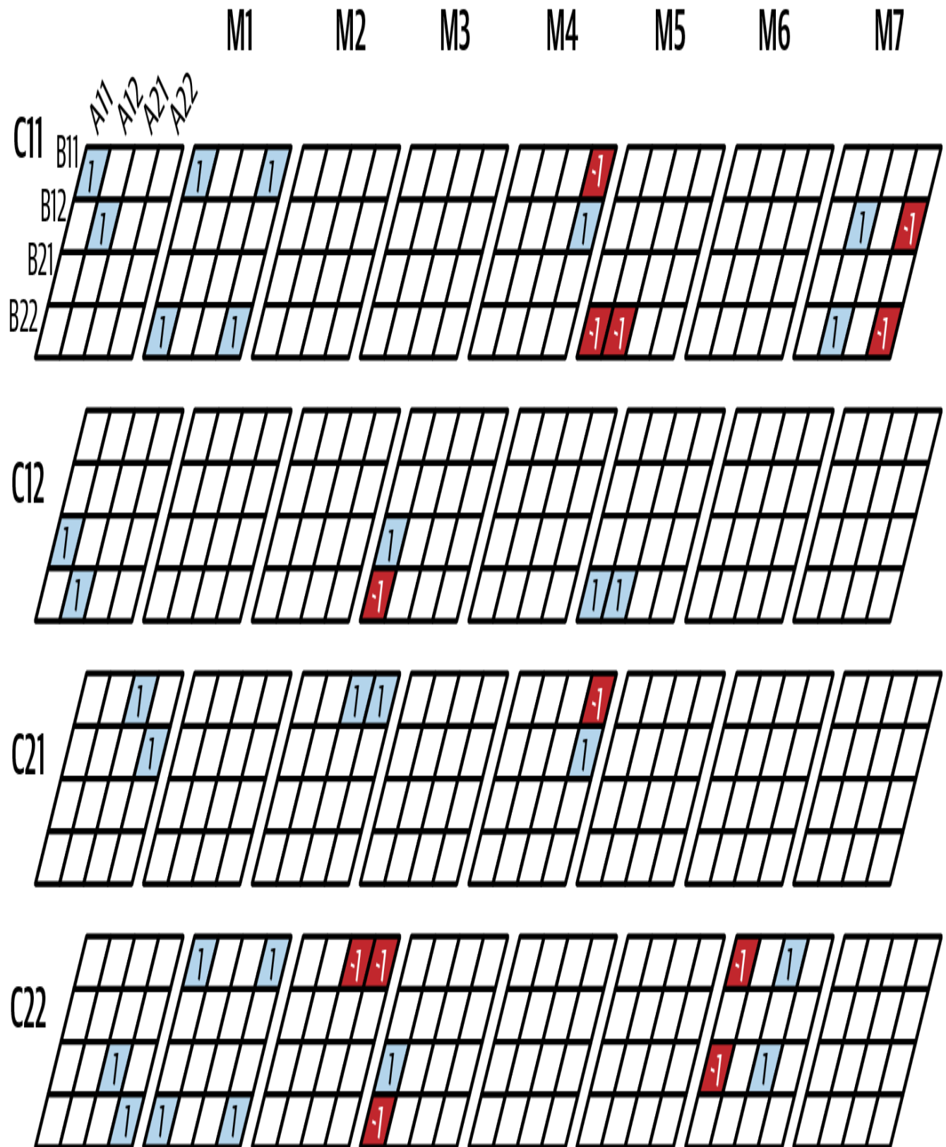
Figure 20-2. Strassen's subquadratic algorithm for multiplying 2 \times 2 matrices (source: https://oreil.ly/5jzLn )
